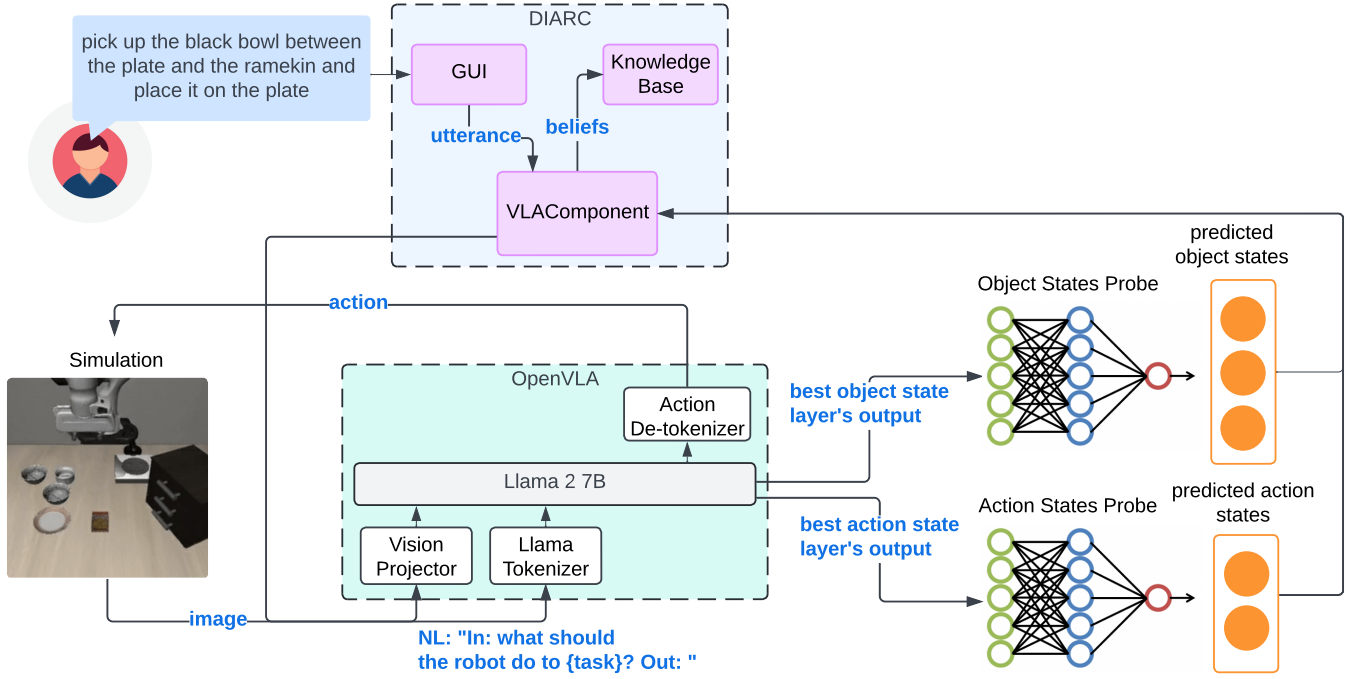
Fig. 1. The DIARC - VLA - Probe System. The user selects a natural language command in DIARC’s Graphical User Interface (GUI). The VLAComponent in DIARC sends this command to OpenVLA. The probes receive two hidden layers’ activations in OpenVLA’s Llama backbone that encode the most object state and action state information respectively. The two best hidden layers are identified through the probing experiment described in Section IV. The probes predict the object state and the action state based on the hidden layers’ activations at each timestep. The VLAComponent in DIARC updates DIARC’s beliefs based on the predicted object state and action state.
