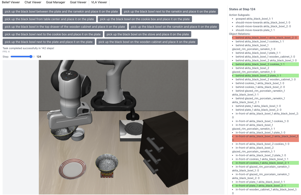
Fig. 2. DIARC-OpenVLA GUI. The left-hand pane displays the real-time camera feed (updated at 5–10 Hz), showing the robot’s manipulation progress. The right-hand pane color-codes each predicted symbolic state (green for newly activated, red for deactivated), letting users quickly verify whether OpenVLA’s internal representation matches the environment. After task completion, a timeline slider appears, allowing the user to revisit earlier steps’ images and states for deeper analysis.
