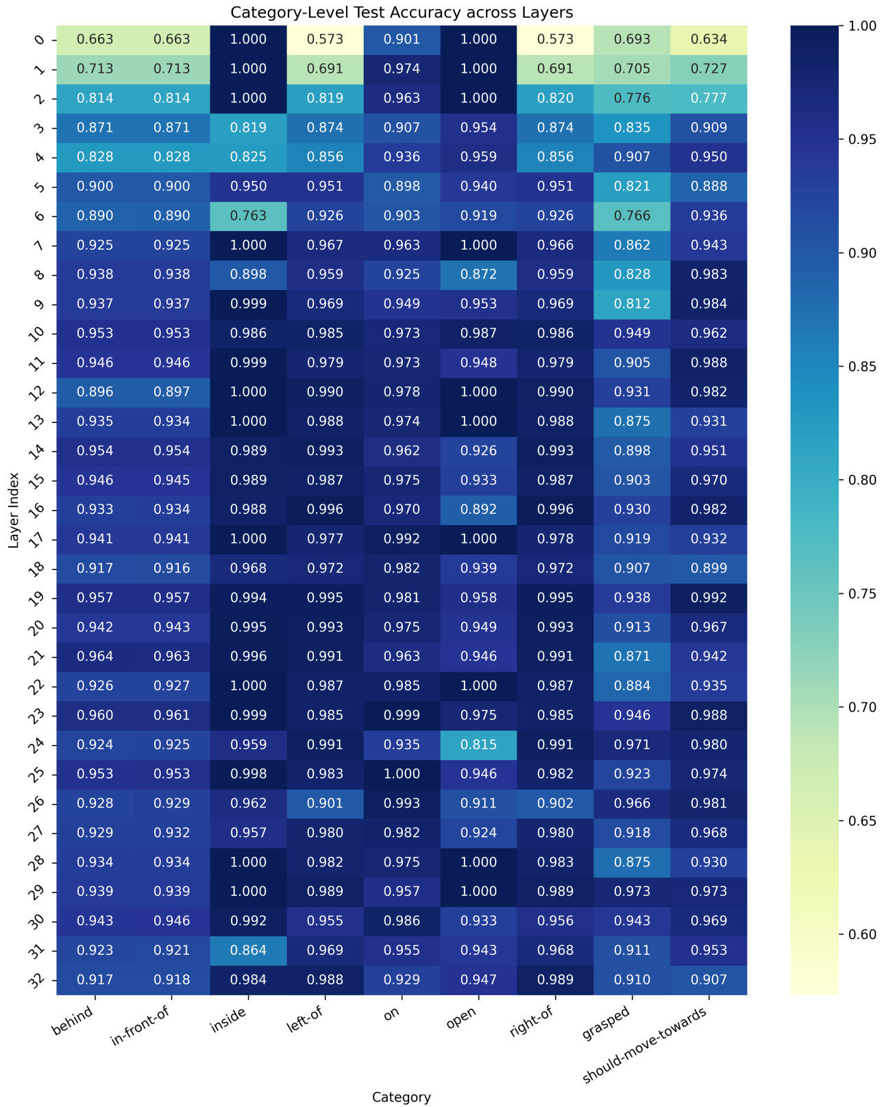
Fig. 4. Probing Results. The first seven columns are object state symbols and the last two columns are action state symbols.
