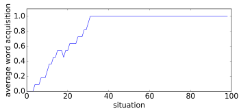
Fig. 2. Average word acquisition score (over time) for all the referential words in the dataset used for sensory noise evaluation (when noise=0). The summary statistics of the lexicon found by the model is precision:0.846, recall:1, F-score:0.916.
