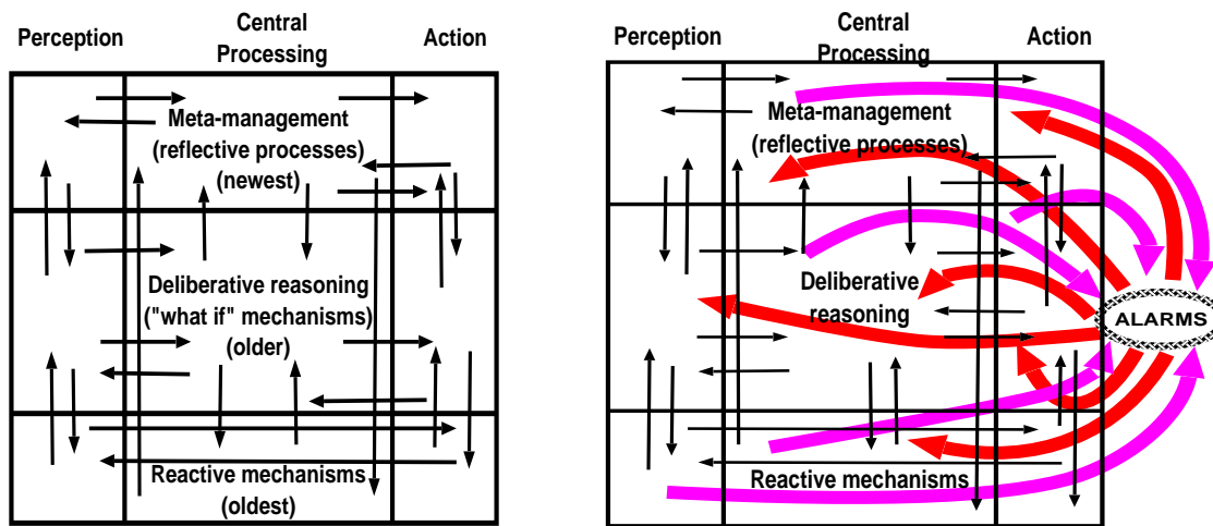
Figure 1: (a) The CogAff architecture schema combines cognitive and affective components. Nilsson's 'triple tower' model, with information flowing (mainly) through perceptual, central, and motor towers, is superimposed on his 'triple layer' model, where different layers, performing tasks of varying abstractness, use different mechanisms and representations. In (a) the two views are superimposed. Components in different boxes have functions defined by their relationships with other parts of the system. In (b) a fast (but possibly stupid) alarm system receives inputs from many components and can send control signals to many components. An insect's architecture might include only the bottom layer. Some animals may have reactive and deliberative layers. Humans seem to have all three. See the text and fig. 2 for details. The diagrams leave out some components (e.g. motive generators) and some information pathways, e.g. 'diagonal' routes.
