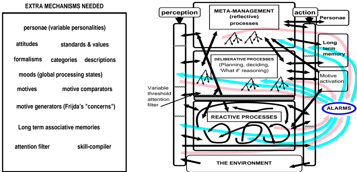
Figure 2: (a) (b) The 'Human-like' sub-schema H-Cogaff. (a) lists some components supporting motive processing and 'what if' reasoning in deliberative and meta-management layers. Humans seem to have all those mechanisms, perhaps organised as in (b), where the alarm system might correspond to the brain's limbic system. An interrupt filter partly protects resource-limited deliberative and reflective processes from excessive diversion and redirection, using a dynamically varying penetration threshold, dependent on the urgency and importance of current tasks – soldiers in battle and footballers don't notice some injuries. Different 'personae' can control processing at different times, e.g. when at home with family, driving a car, interacting with subordinates, in the pub with friends, etc. Such an architecture has various kinds of information stores, and diverse information routes through the system, only a subset of which are shown.
