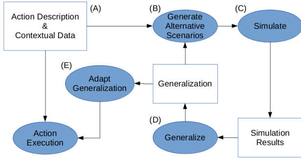
Figure 2: The action generalization process. The letters correspond to the subsections below and depict the typical data flow.
