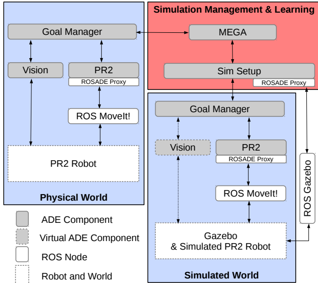
Figure 5: High-level view of the integrated architecture. The blue computational groups represent partial architecture configurations for the physical robot (left) and simulated robot (right). The salmon colored group contains novel algorithms for generalization through analogical reasoning.
